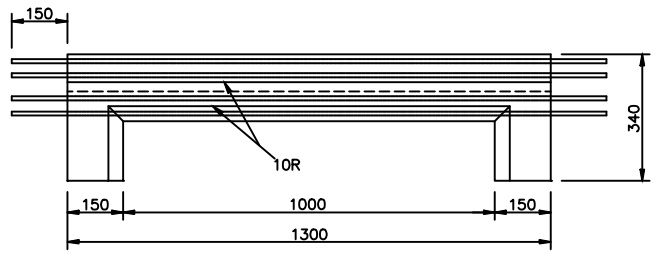
FRONT ELEVATION
