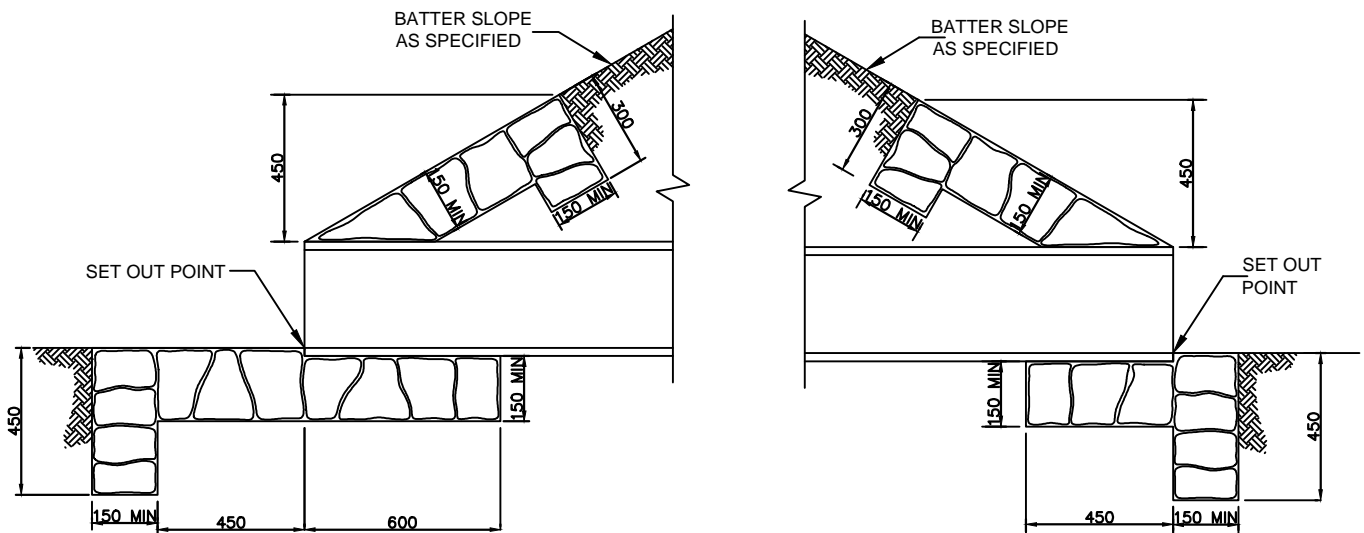
OUTLET SECTION
