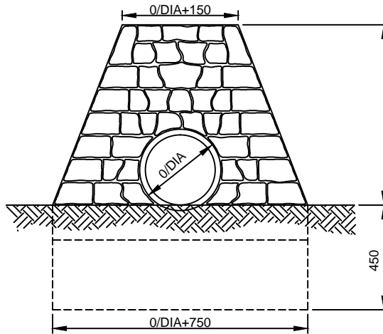
INLET AND OUTLET END ELEVATION
